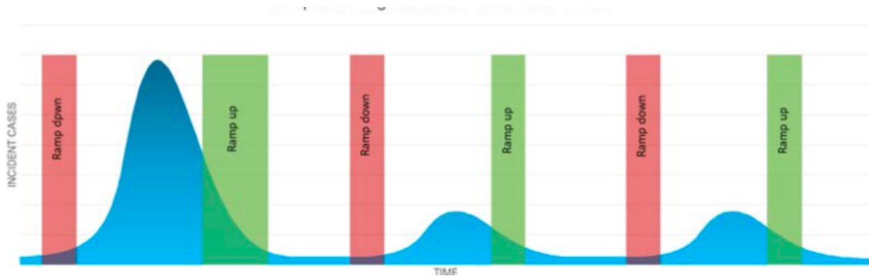
Sample of expected pandemic curve, included epi-curves
